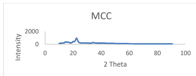
Figure 6. The XRD spectrum for MCC
