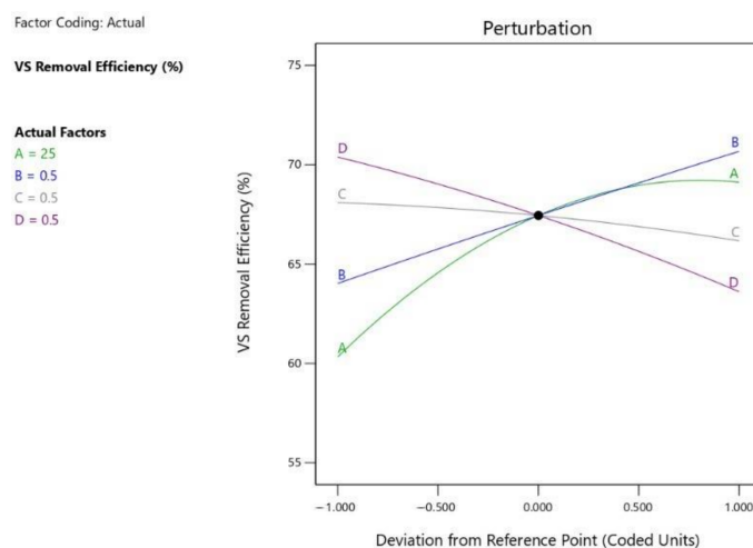
Figure 6. Perturbation plots for VS removal efficiency response.
