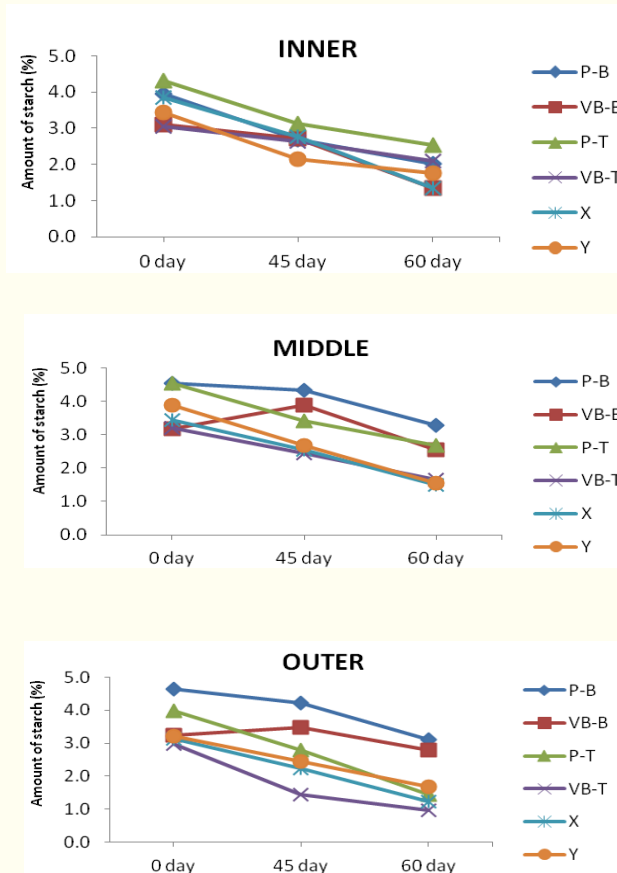
Figure 6 Amount of starch content at different part of the oil palm trunk during storage time
