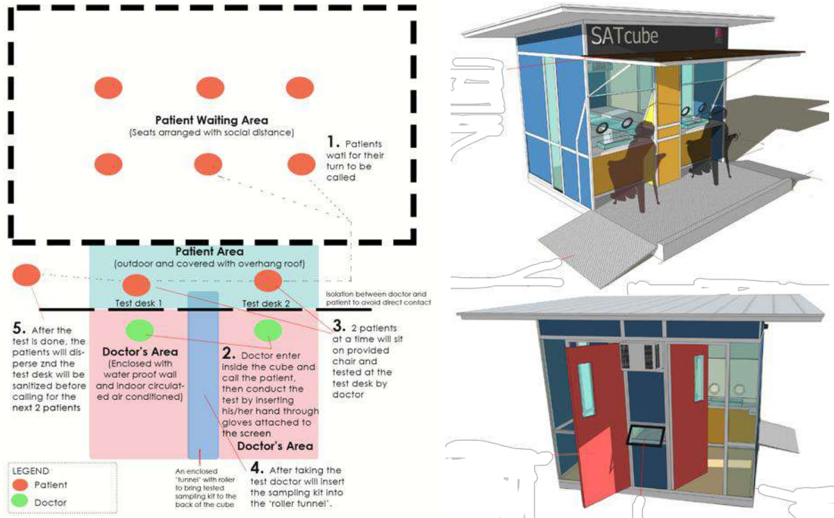
Figure 1: Spatial organisation, the sampling operational and the outer look of the S.A.T Cube
