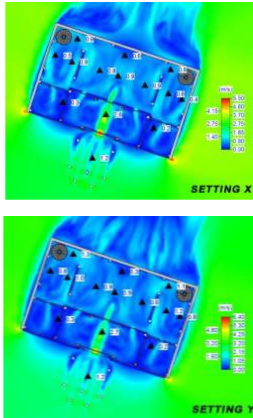
Fig. 2 CFD Simulation of the Ground Floor for wind flow from the South-Southwest
