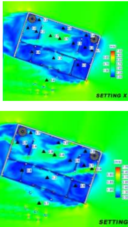
Figure 4 CFD Simulation of the Ground Floor for wind flow from the East
