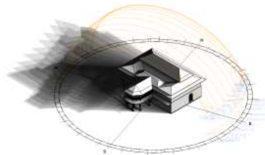
Fig. 7 Shadow range during sunrise for the year 2015
