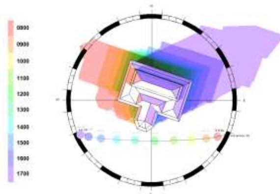
Fig. 8 Solar path and shadow projection range during the winter solstice
