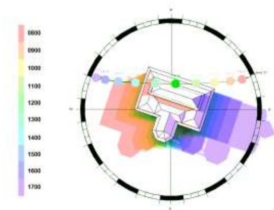
Fig.10 Solar path and shadow projection range during the summer solstice
