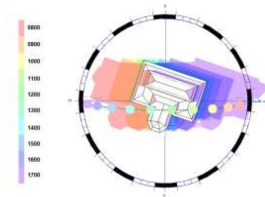
Fig. 9 Solar path and shadow projection range during the vernal equinox
