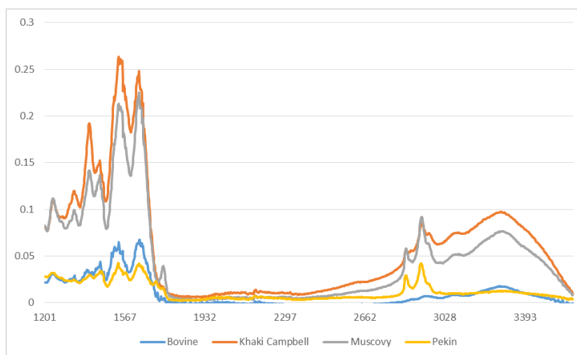
Figure 2 : FTIR spectra of commercial bovine gelatin (CBG) and four different species of duck feet gelatin (DFG)
